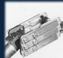
CBV 23kV, 1200A Contact
